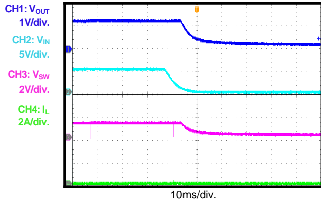
V_{IN} Shutdown
