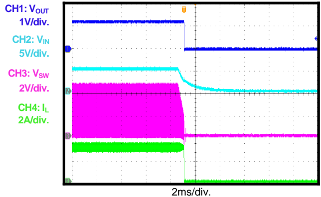
V_{IN} Shutdown
