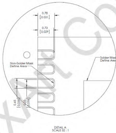
Figure 14. Recommended PCB Layout in mm [inch]
