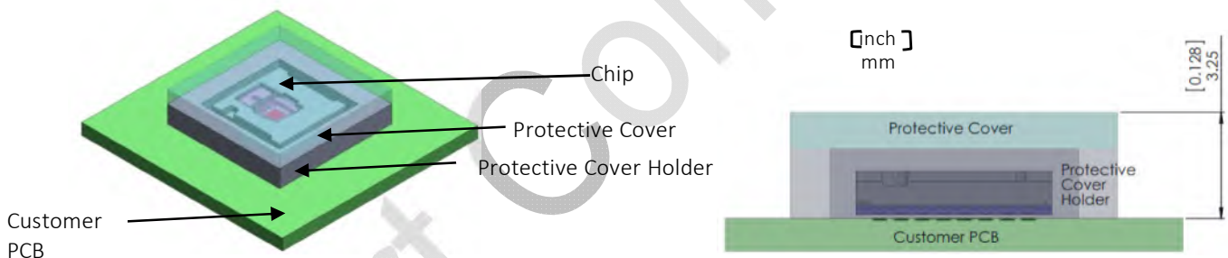
Figure 17. Chip with Flat Cover and Side View
