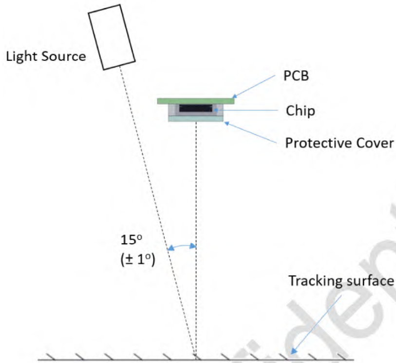
Figure 5. Test setup under bright ambient light
