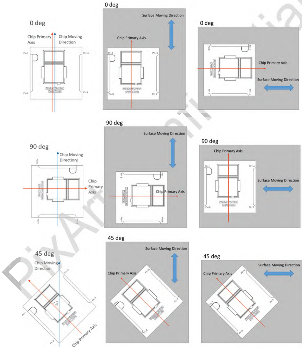
Figure 3. Chip Orientation vs Moving Direction
