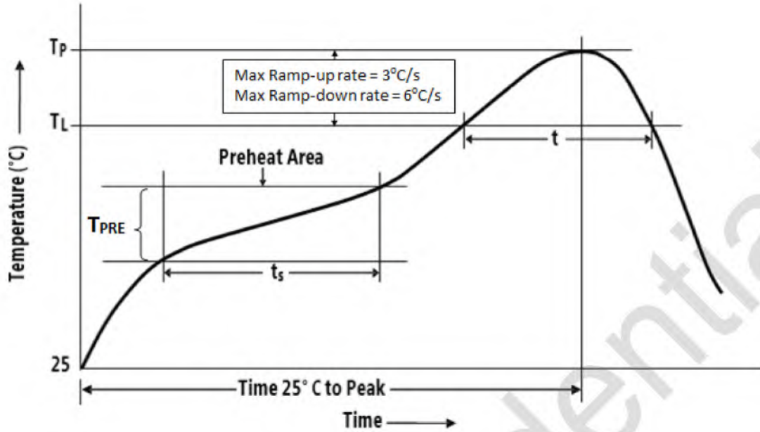
Figure 21. Soldering Reflow Profile
