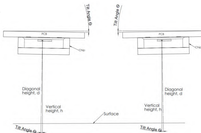
Figure 15. Tilt Definition
