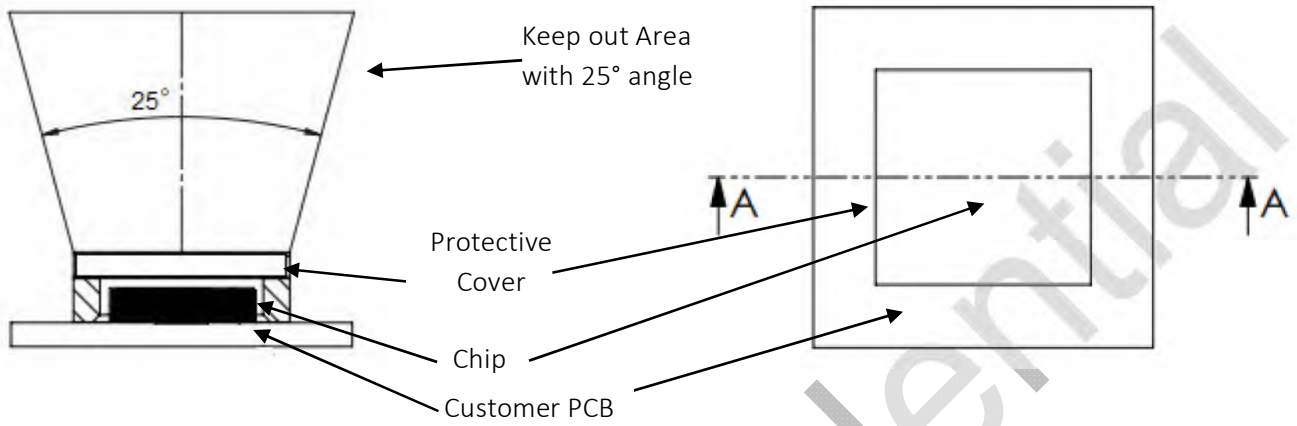
Figure 16. Side View and Top View of Keep out Area
