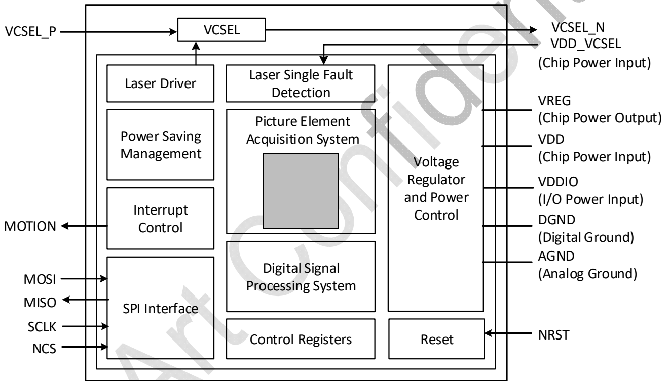
Figure 1. Block Diagram
