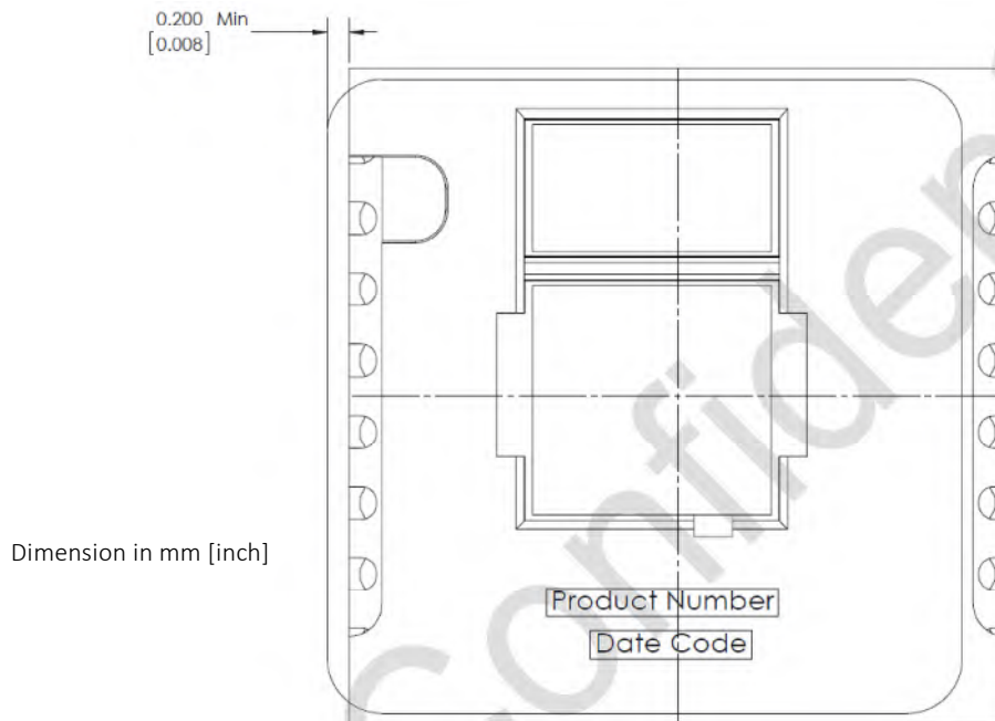
Figure 19. Kapton Tape Offset Position
