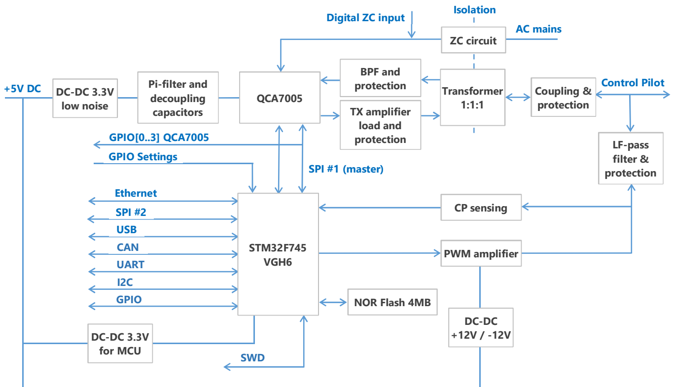
FIGURE 3-1. WHITE-BEET-E (EVSE) BLOCK DIAGRAM
