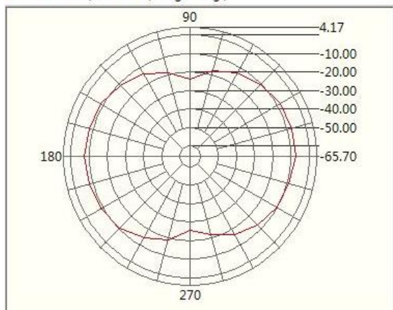
1.71GHzRight-Left
