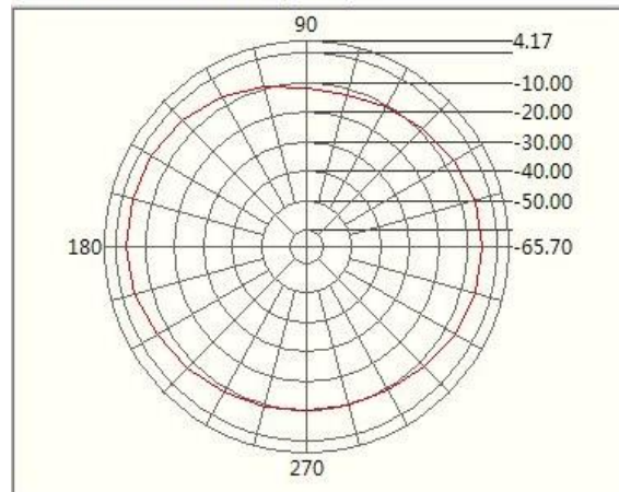
1.71GHz@Theta
