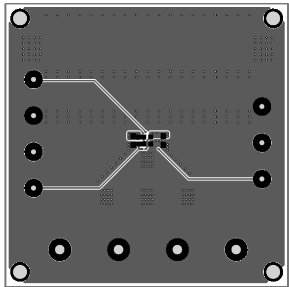
Figure 4: Bottom Layer
