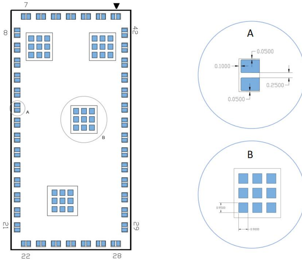
Figure 6 – Recommended Solder Paste Footprint
