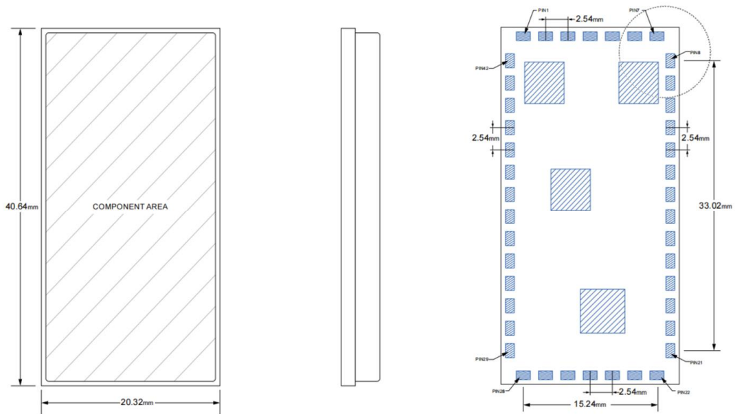
Figure 4 – DB2605 Form Factor
