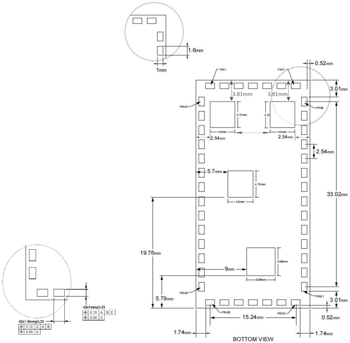
Figure 5 – Recommended Footprint
