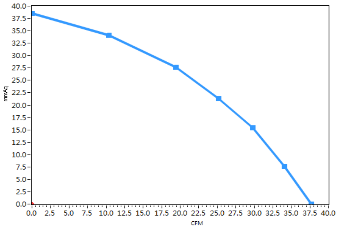
P-Q Curve
